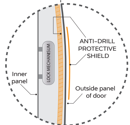
CROSS SECTION OF PROTECTION SHIELD
